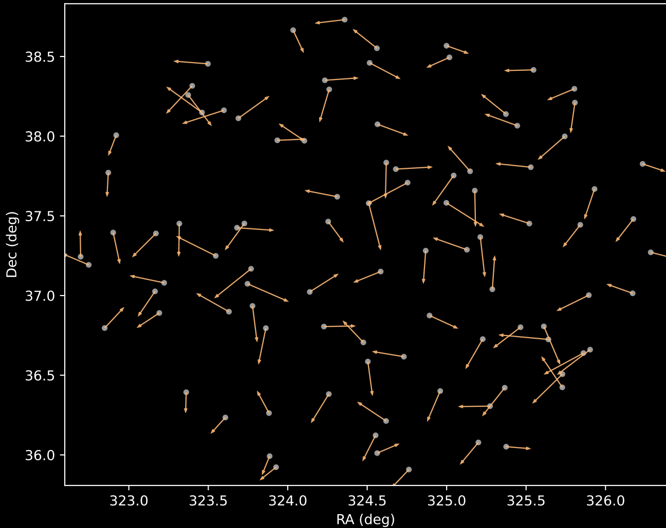
APOGEE DR17 Cluster 3 Proper Motion Vectors (n=95)
