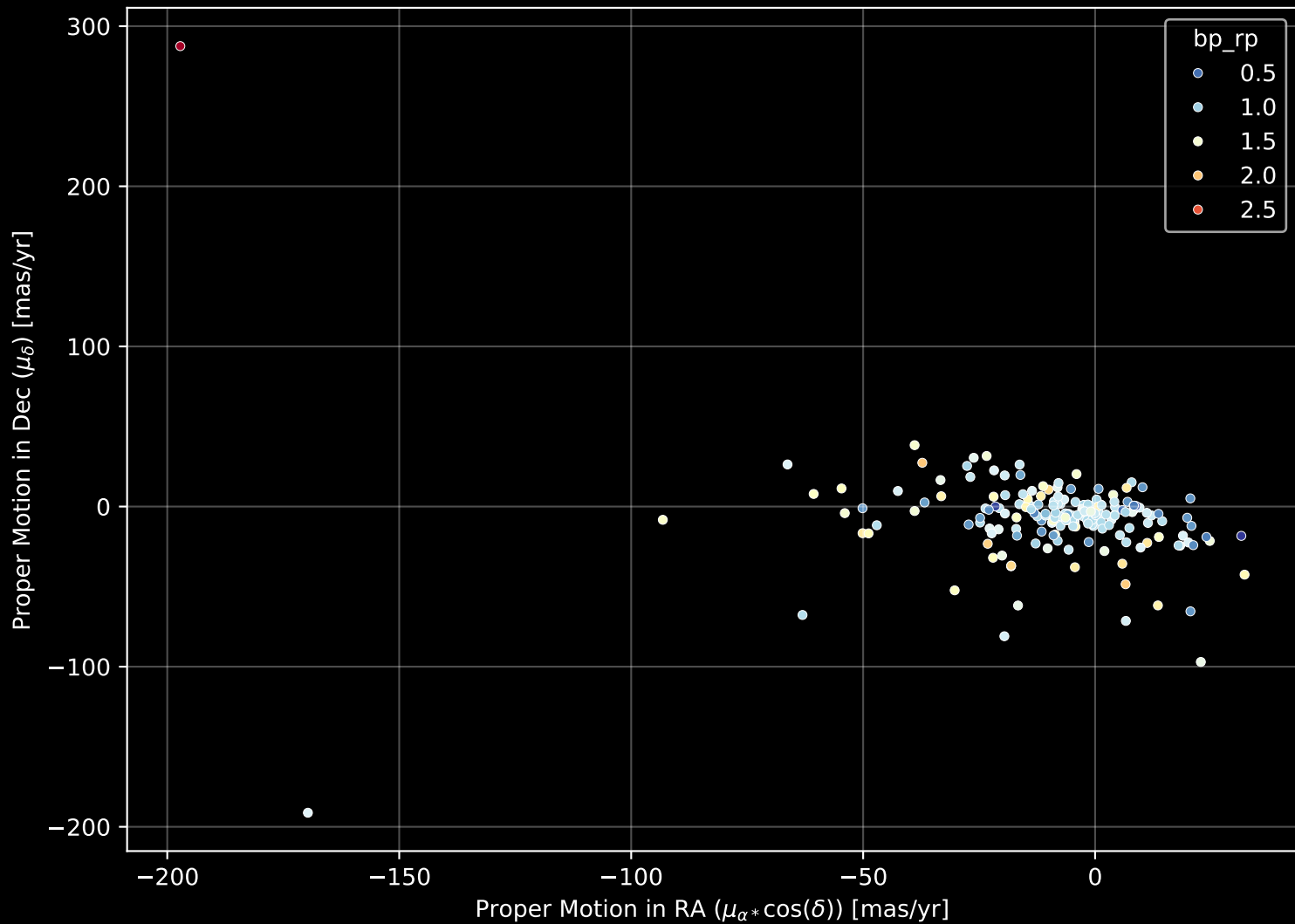
APOGEE DR17 Field: [062+62] Proper Motion Diagram (n= 187)
