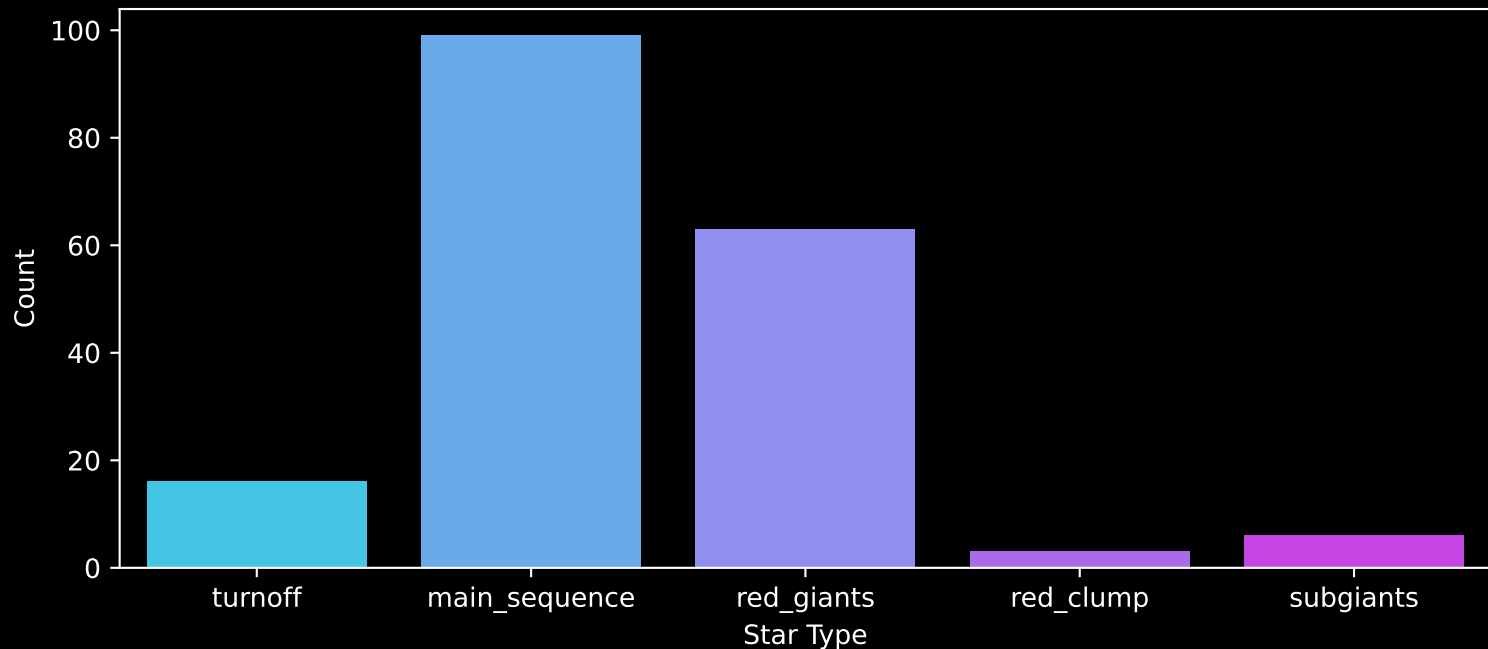
APOGEE DR17 Field: [062+62] Count plot of Star Type
