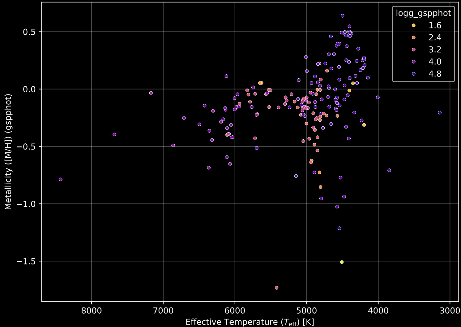
APOGEE DR17 Field: [062+62] Stellar Population Parameters (n= 187)
