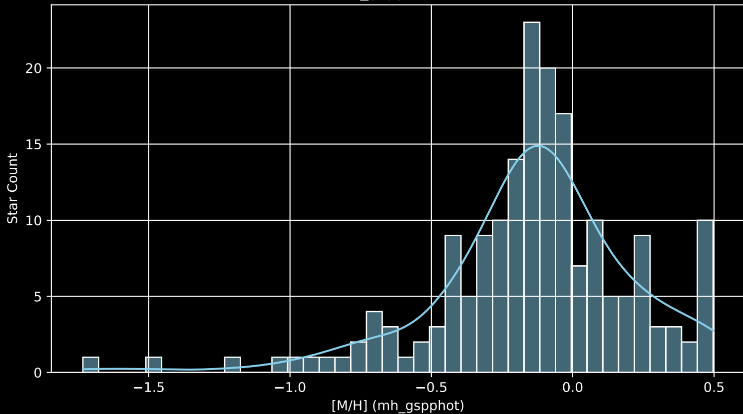
APOGEE DR17 Field: [062+62 [M/H] (mh_gspphot) (n= 184)
