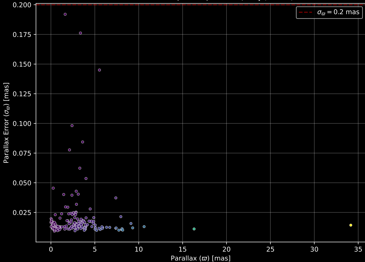
APOGEE DR17 Field: [062+62] Parallax Quality (n= 187)
