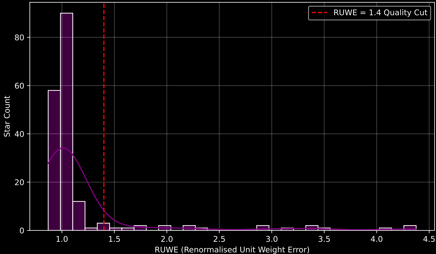
GAPOGEE DR17 Field [062+62] RUWE Distribution (n= 182)
